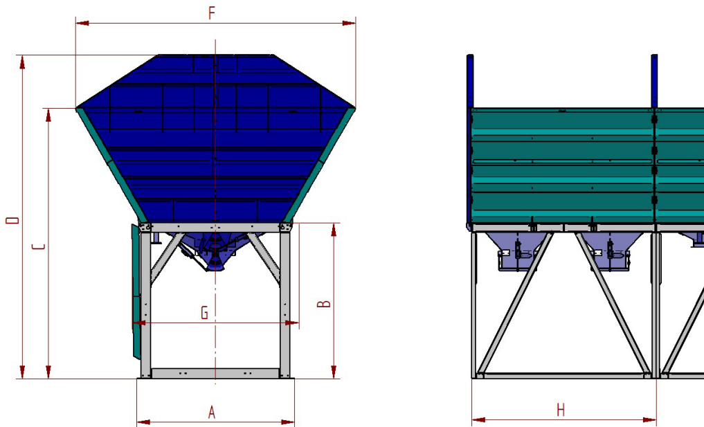
Dimensions of one single compartment of RD 35
